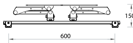
Order Code PLA2X1 Fits VESA 300 x 300 to 600 x 400 £ Ex Vat 288.10 (Comes with Pozimount PZX1)
